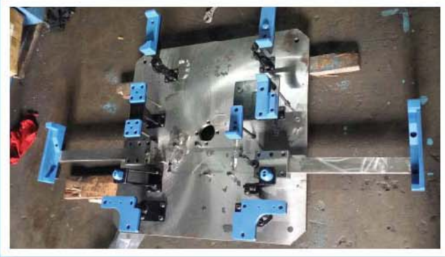
● Front Suspension Pallet Tray
